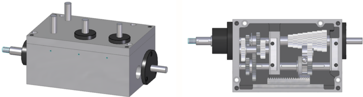
Norton Gearbox for Lathe
