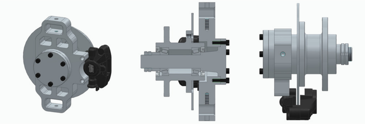
FSAE Supra - Front Wheel Assembly
